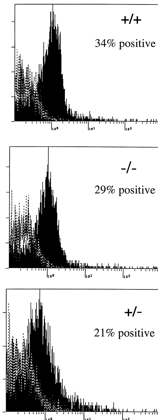
Fig. 5. TWEAK binds to both murine wild-type and WSL-1/TRAMP knockout cells. Peripheral blood lymphocytes from wild-type and wsl-1 knockout mice were incubated for 10 min in the presence or absence of FLAG-tagged murine TWEAK (3 \mu g). Cells were then incubated with 0.5 \mu g anti-FLAG conjugated to biotin, following the blocking of murine Fc receptors with normal mouse serum. Finally the cells were incubated with 0.5 \mu g Streptavidin Alexa488, washed in FACS buffer and analysed by flow cytometry.
